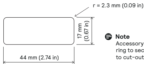
Cut-out in metal sheet (max. thickness 0.7 mm to 1.2 mm)
